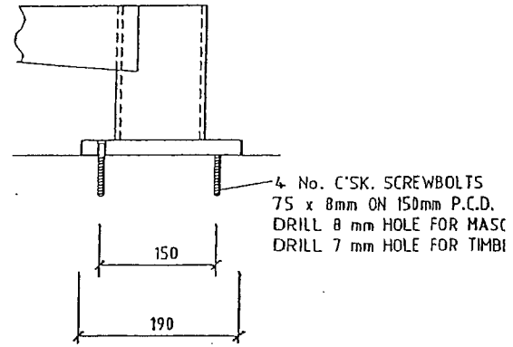
Base Plate
