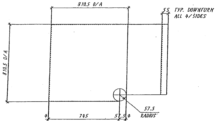
LANDING DETAIL
